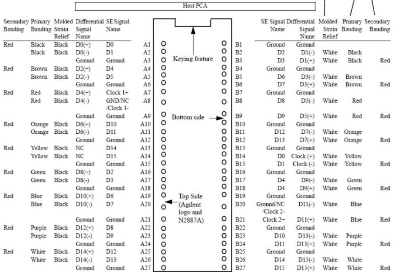
N2887A Soft Touch Pro-to-InfiniiMax Adapter Pin-Out
