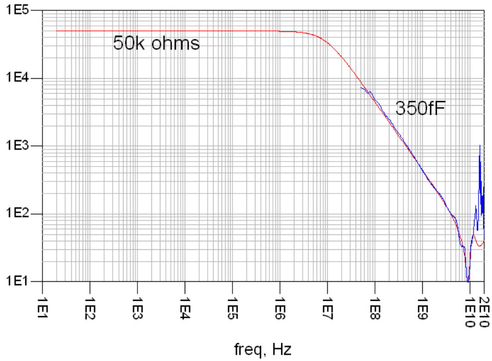
Differential input impedance (red = model, blue = measured)
