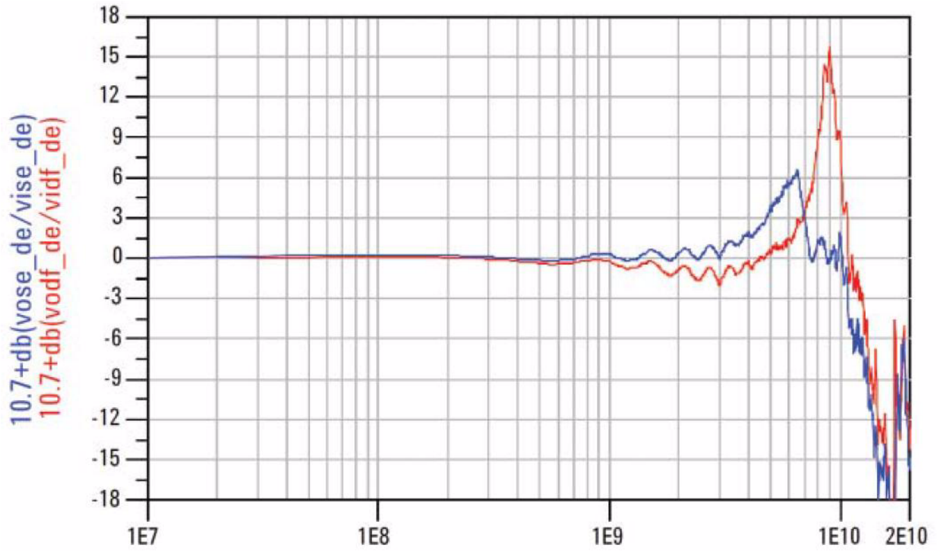
Frequency response, N2887A with an 1169A 12 GHz amplifier (red = differential, blue = single-ended)
