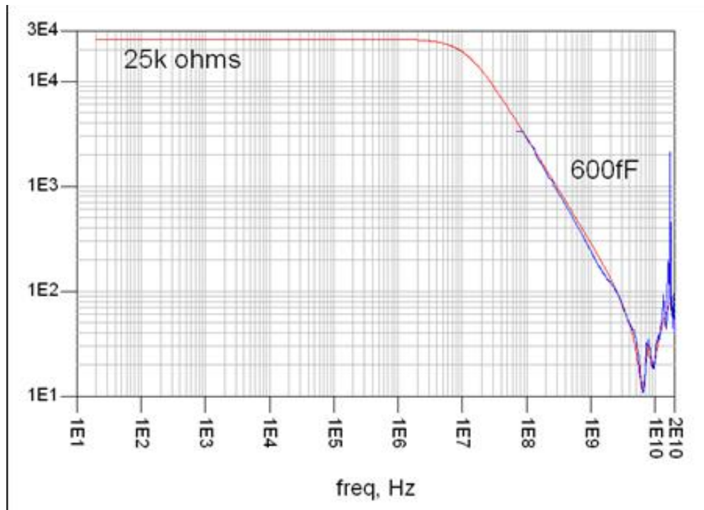
Single-ended input impedance (red = model, blue = measured)
